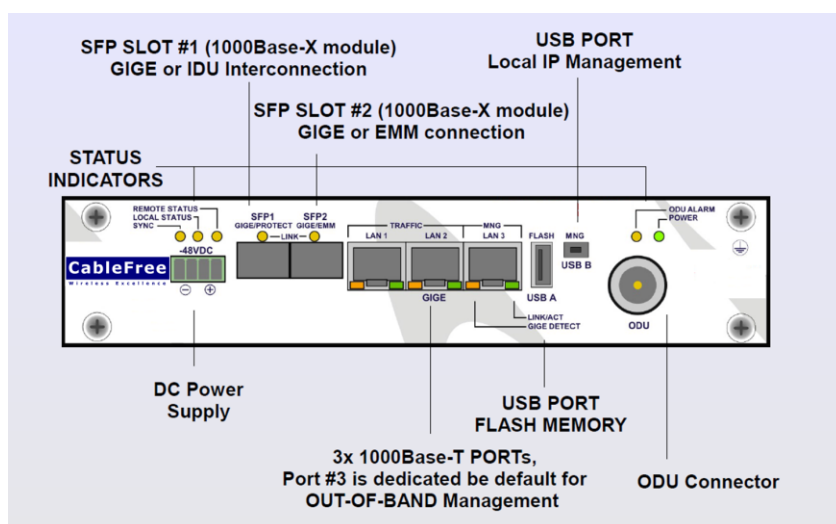
Above: Microwave Modem and IP Interface Module
